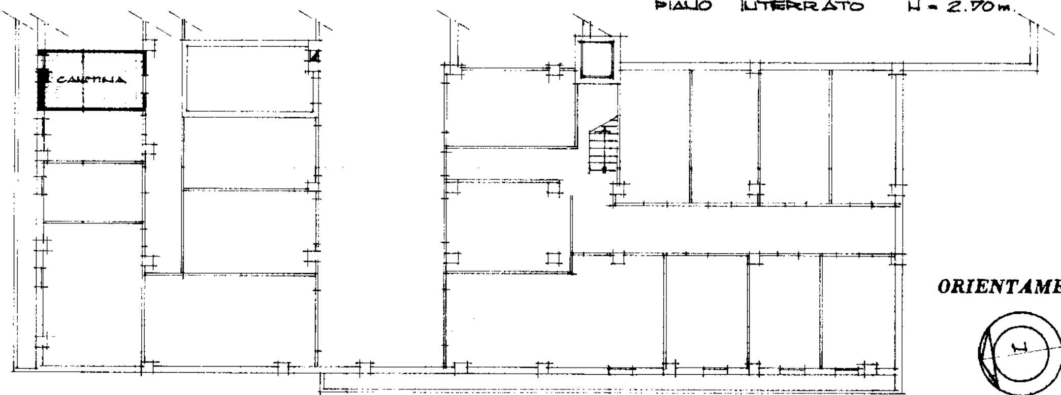
PIANO INTERRATO H = 2.70m.
